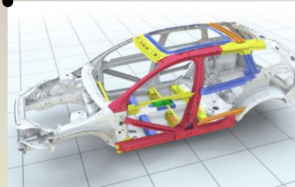
1991 Side Impact Protection System (SIPS)
